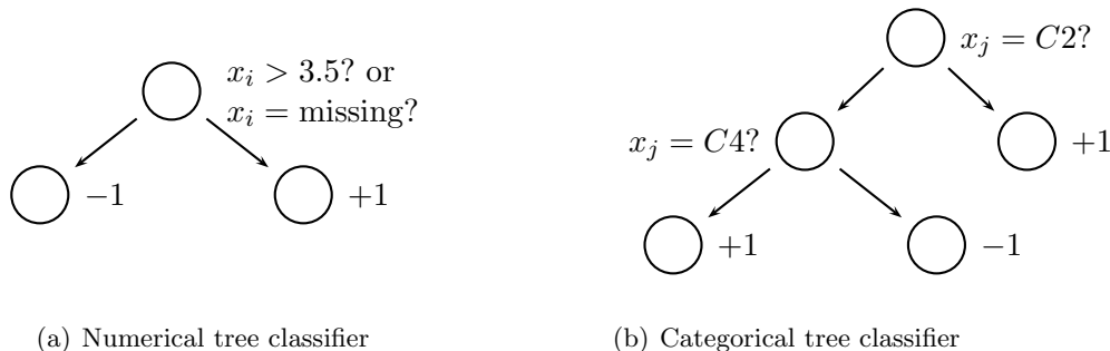
Figure 1: Example of numerical and categorical tree classifiers
